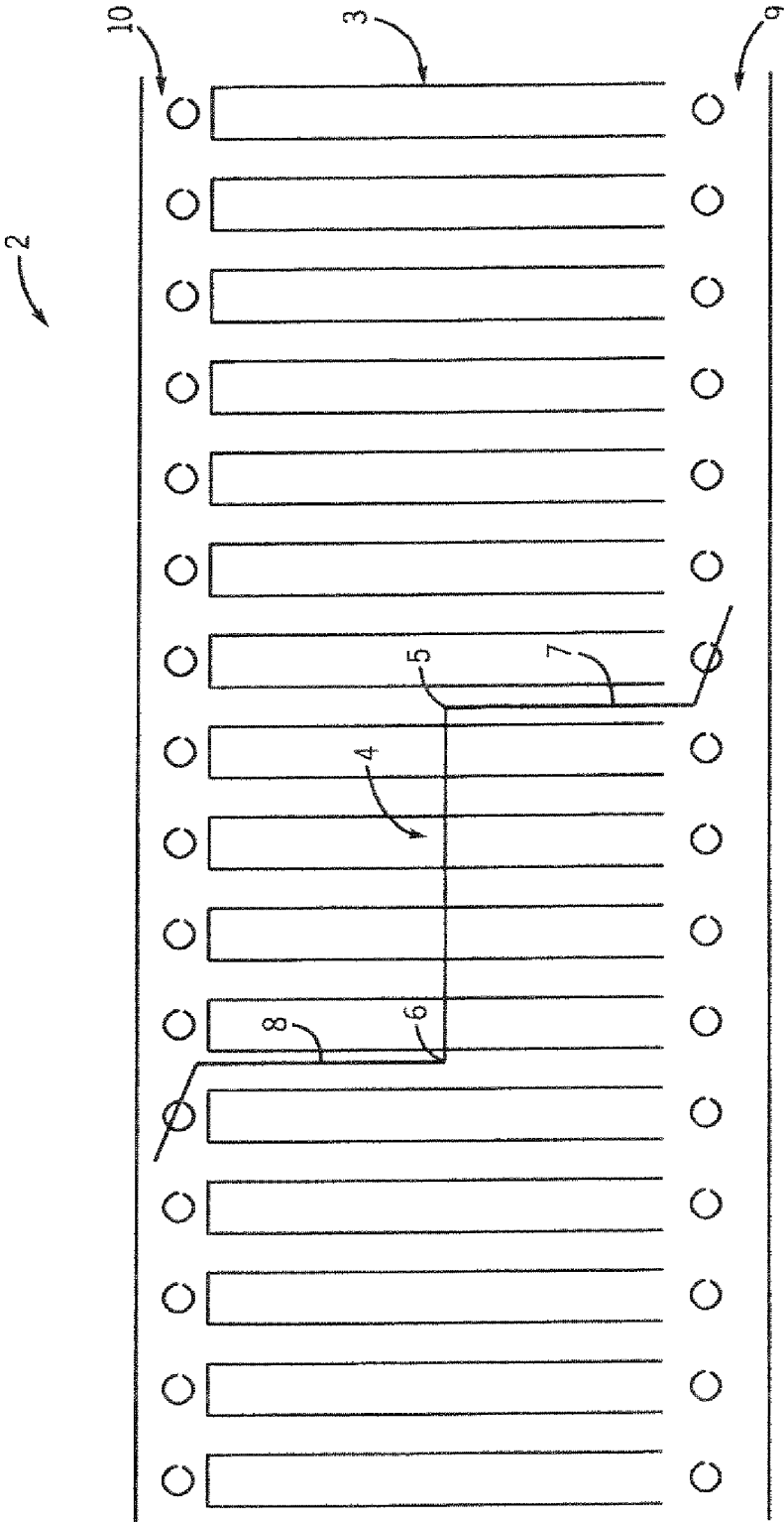
FIG. 1 PRIOR ART
