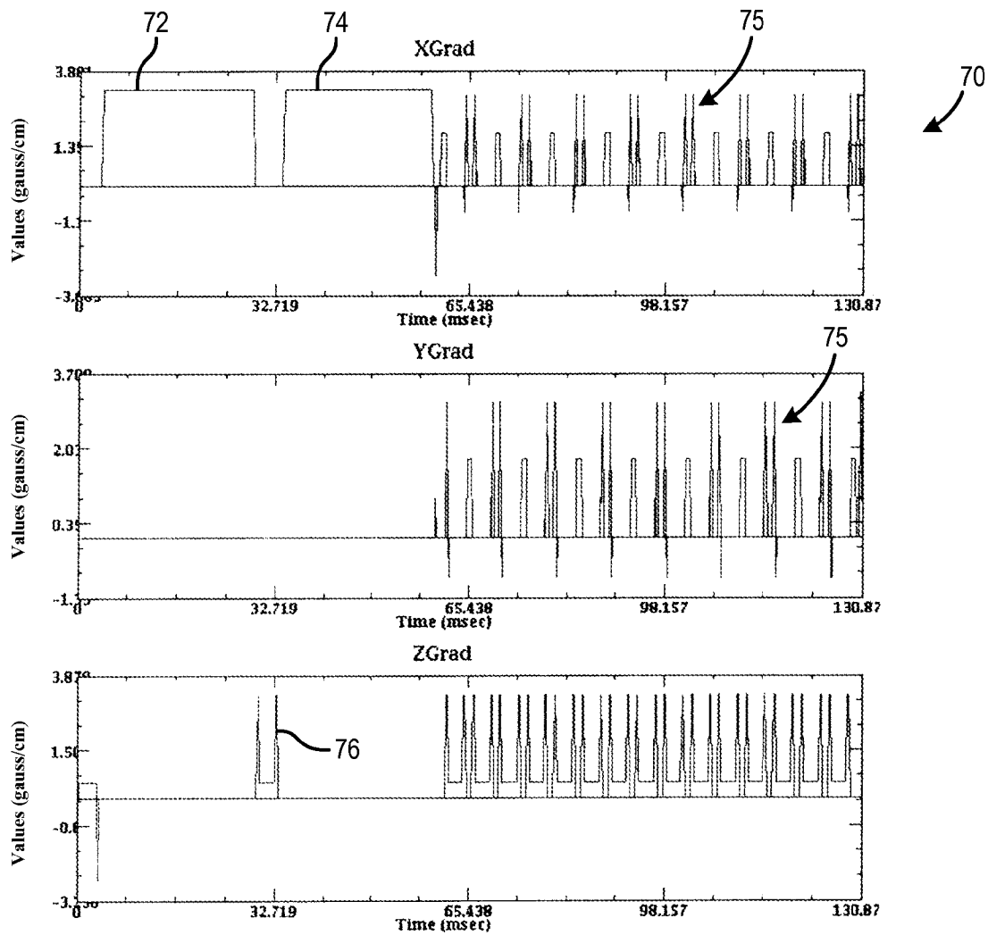
FIG. 2 -PRIOR ART-
