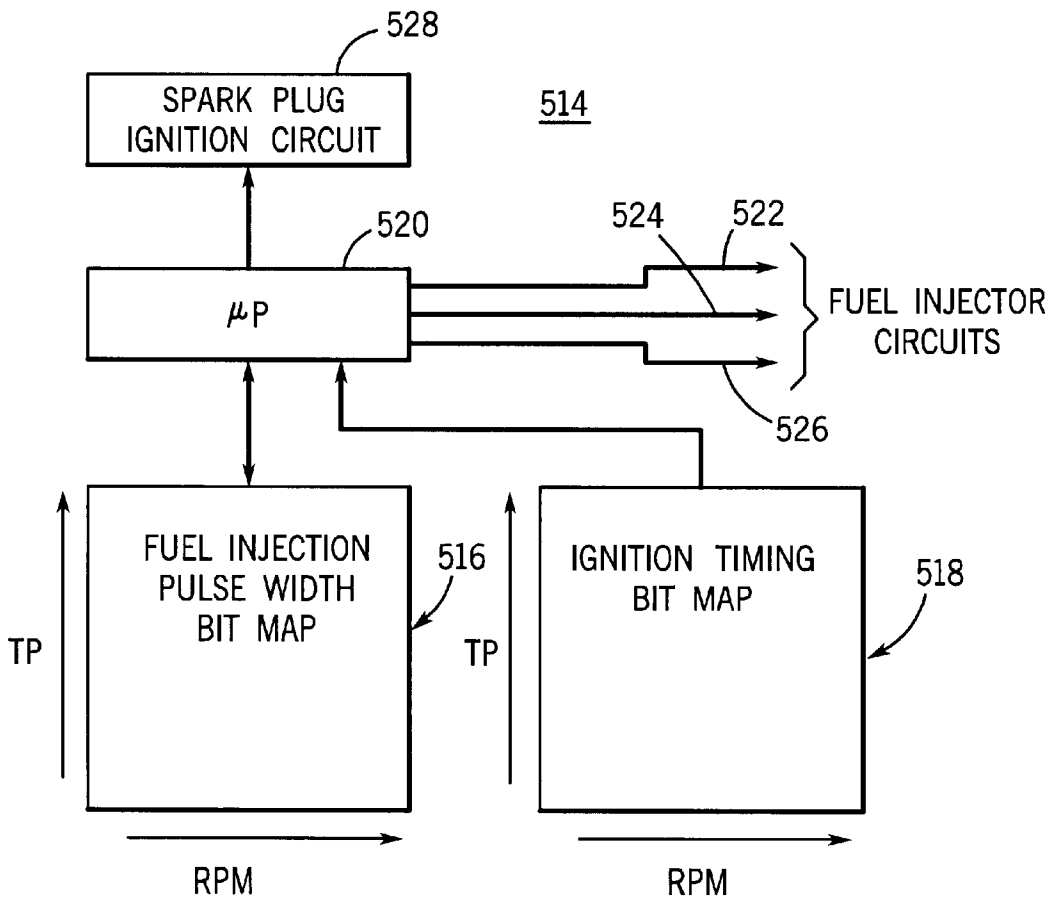
FIG. 7 (PRIOR ART)
